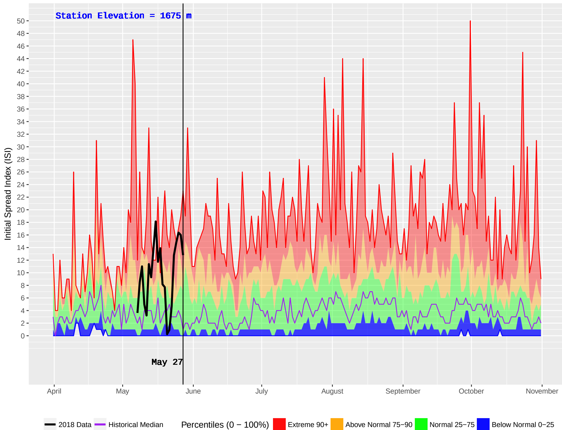
GASPARD (222) : Historical (1992–2016) and Current (2018) Noon Initial Spread Index (ISI)
