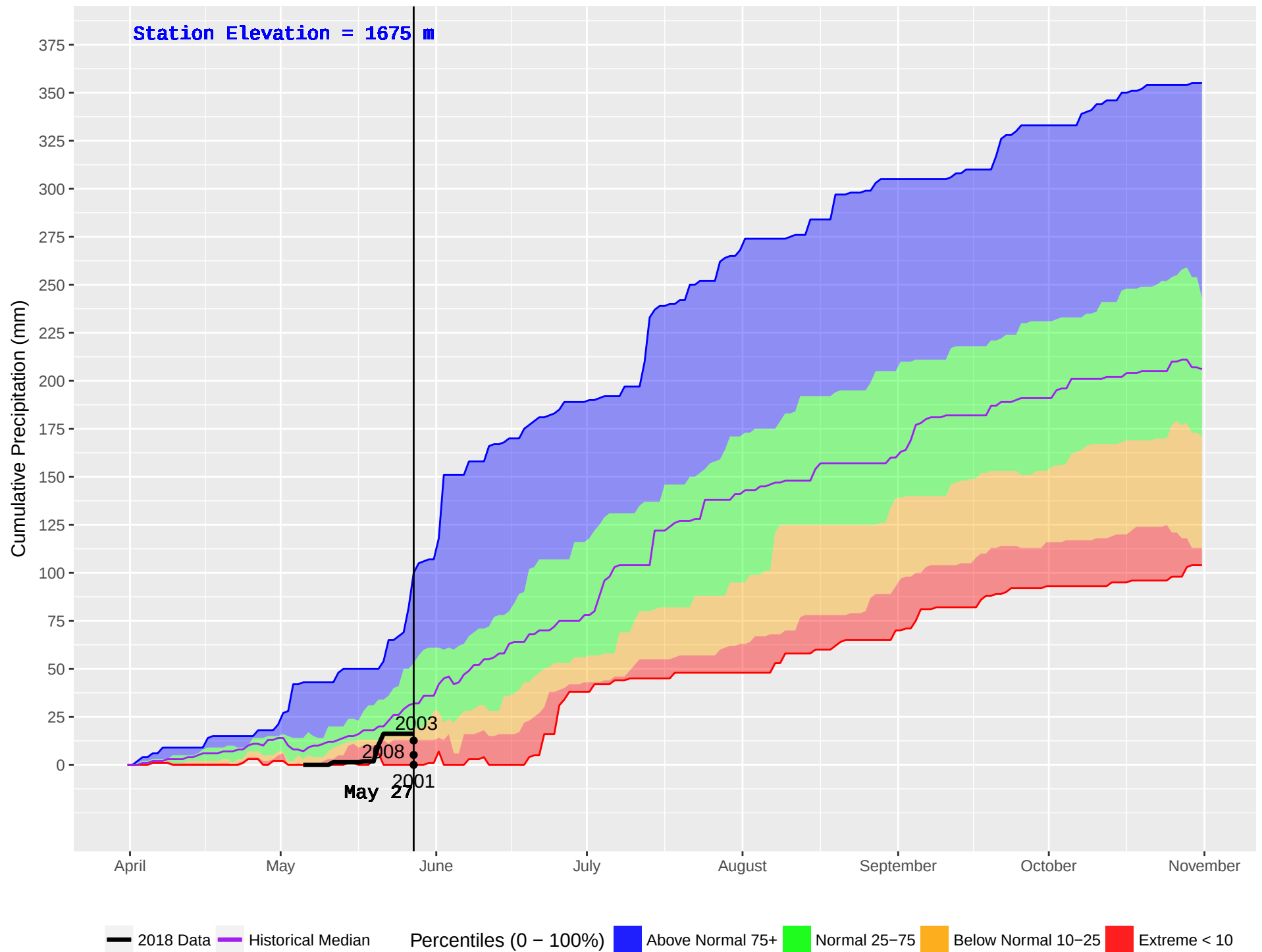
GASPARD (222) : Historical (1992–2016) and Current (2018) Noon Cumulative Precipitation
