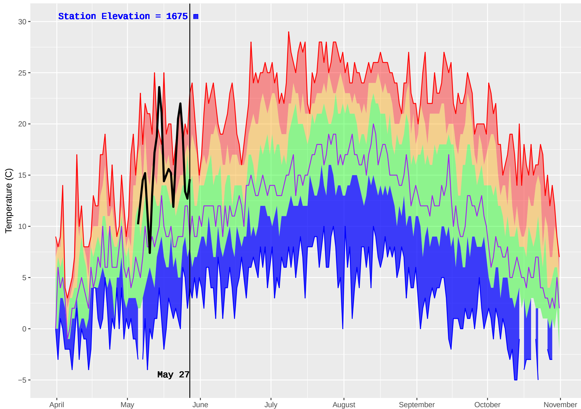
GASPARD (222) : Historical (1992–2016) and Current (2018) Noon Temperature
