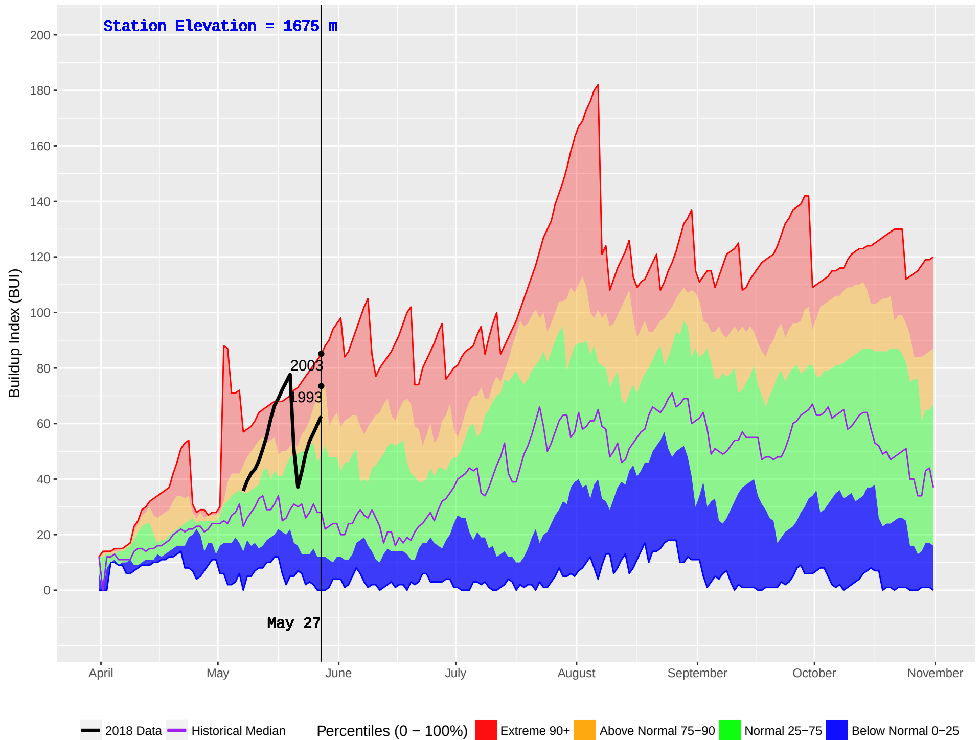
GASPARD (222) : Historical (1992–2016) and Current (2018) Noon Buildup Index (BUI)
