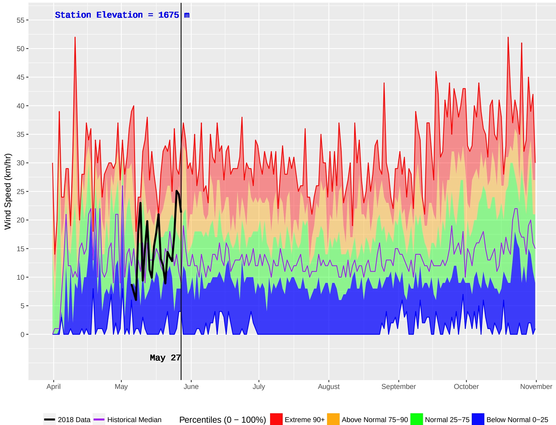
GASPARD (222) : Historical (1992–2016) and Current (2018) Noon Wind Speed
