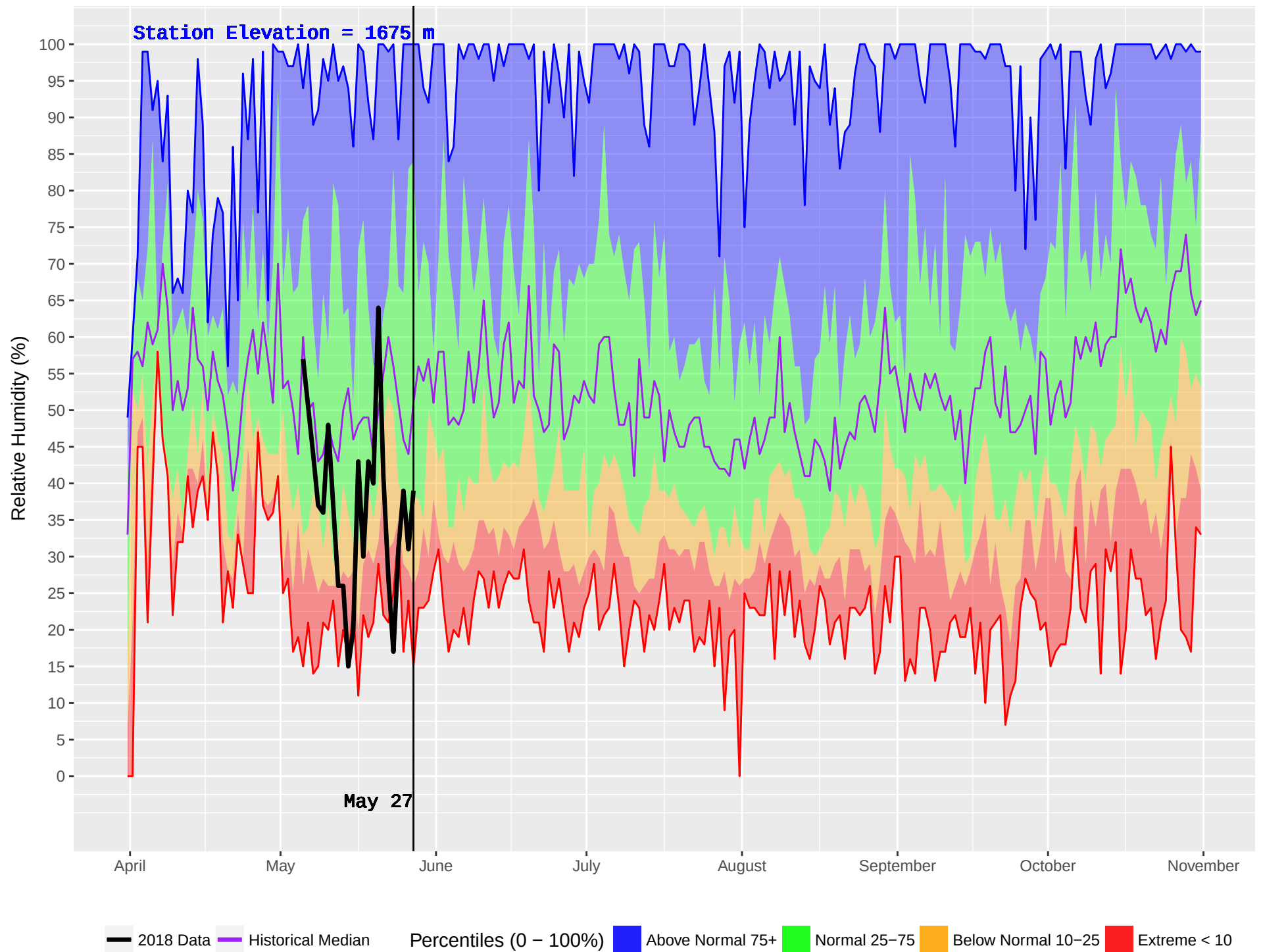
GASPARD (222) : Historical (1992–2016) and Current (2018) Noon Relative Humidity
