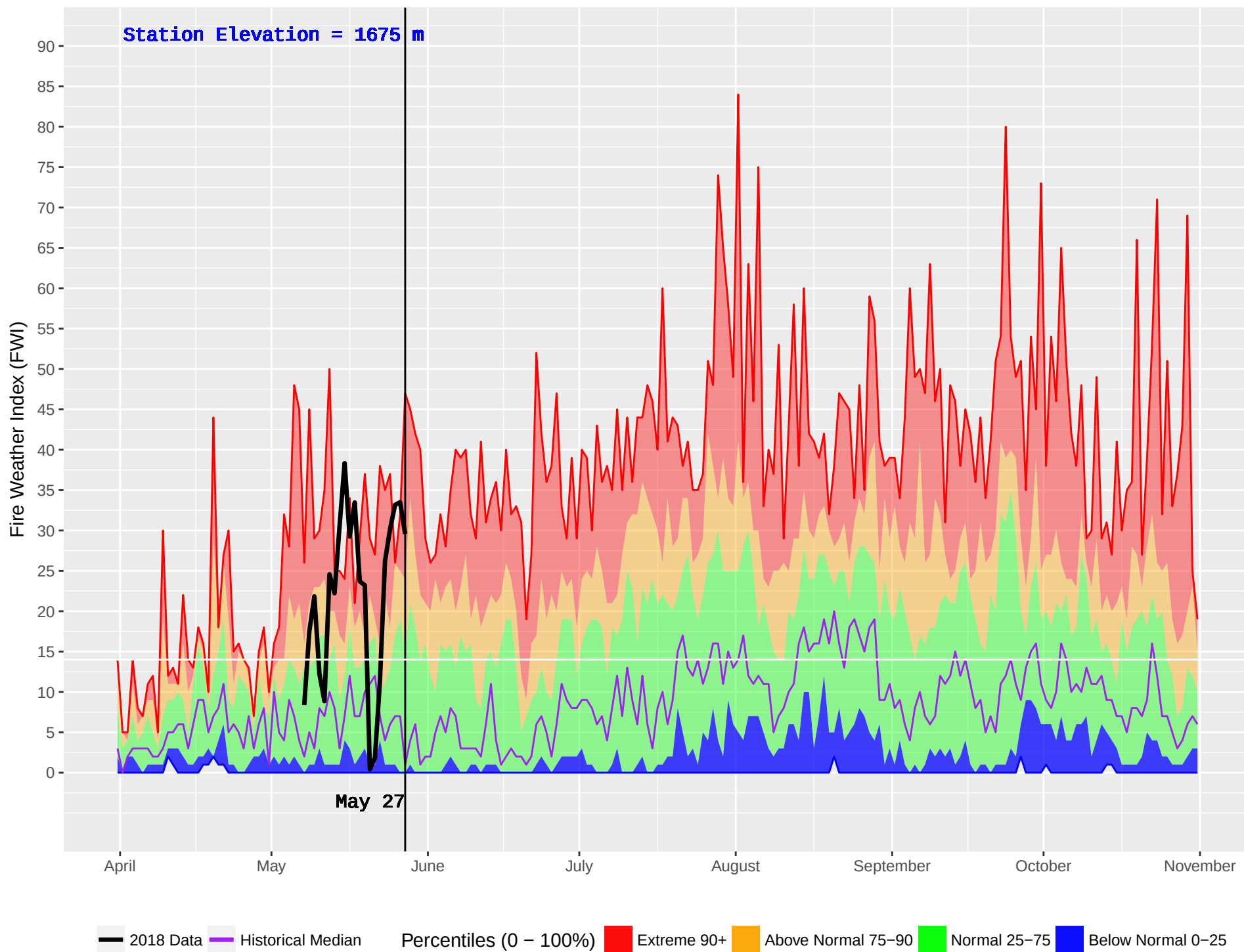
GASPARD (222) : Historical (1992–2016) and Current (2018) Noon Fire Weather Index (FWI)
