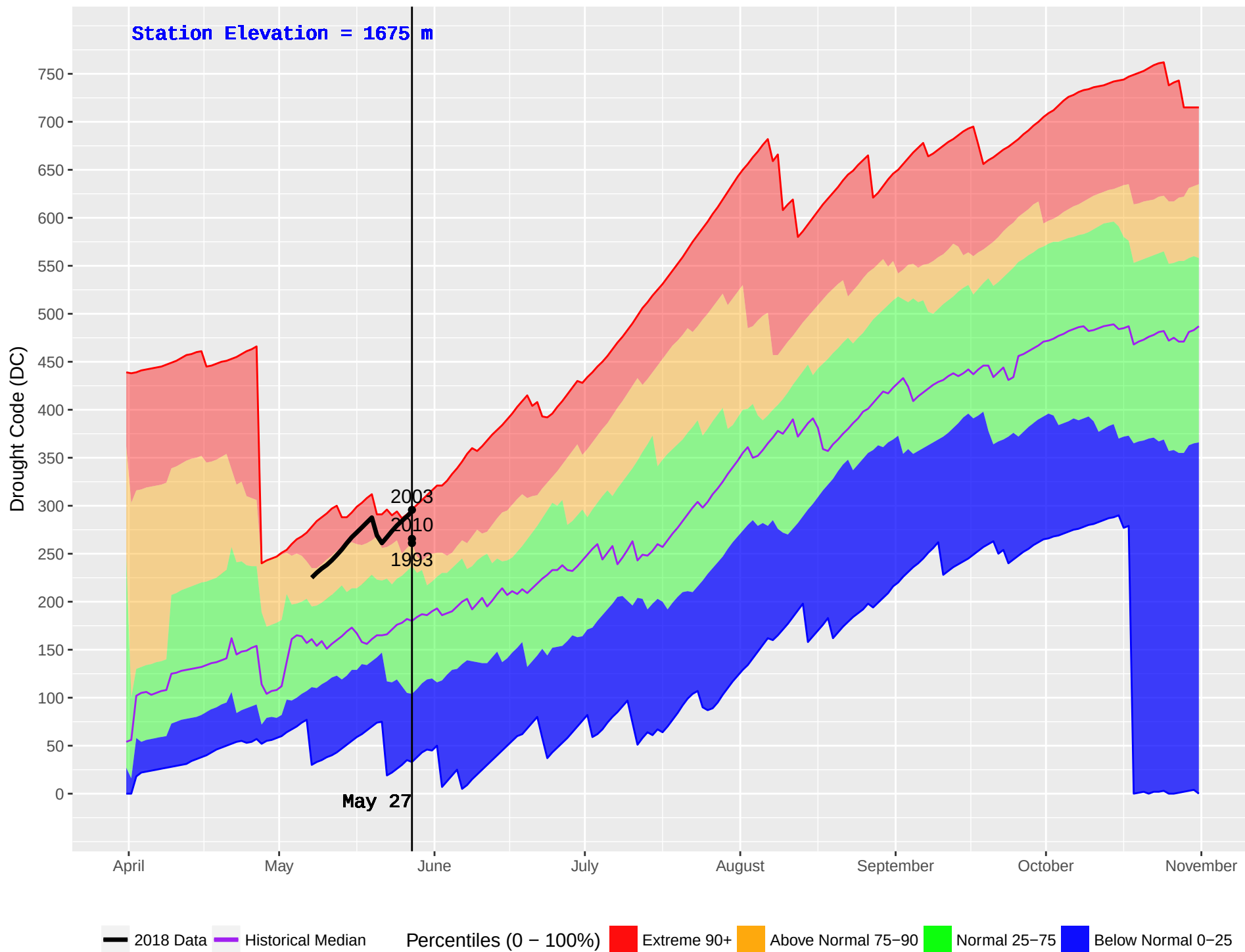
GASPARD (222) : Historical (1992–2016) and Current (2018) Noon Drought Code (DC)
